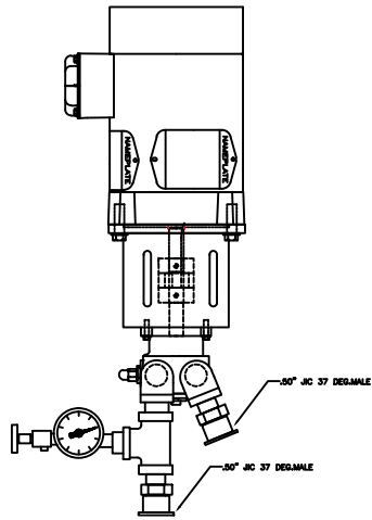
ASSEMBLY MOUNTING ARRANGEMENT WITH SS FITTINGS PACKAGE
