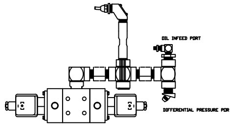
SOLENOID & FLOW SENSOR ARRAY
